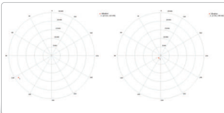
► Figure 8. Rotor vibration vector before (left) and after (right) balancing
