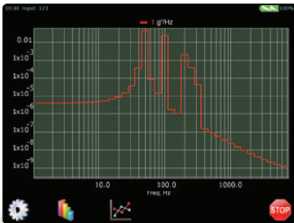
► Figure 5. 1/3-octave spectrogram
